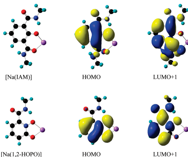
FIGURE 12. Results from TD-DFT (B3LYP/6-311G ++ (d,p) for simplified model [Na(IAM)] (top) and [Na(1,2-HOPO)] (bottom) chromophores, revealing the \pi \rightarrow \pi^* character of the low-lying excited singlet and triplet states.
