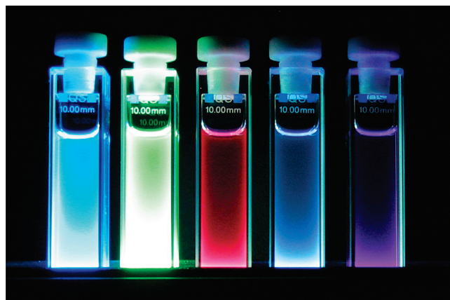
FIGURE 8. Observed emission from Ln(III) cations sensitized by an IAM ligand irradiated with a standard laboratory UV lamp ( \lambda_{\text{ex}} = 365\text{ nm} ). From left to right, ligand only, Tb(III), Eu(III), Dy(III), and Sm(III) complexes.
