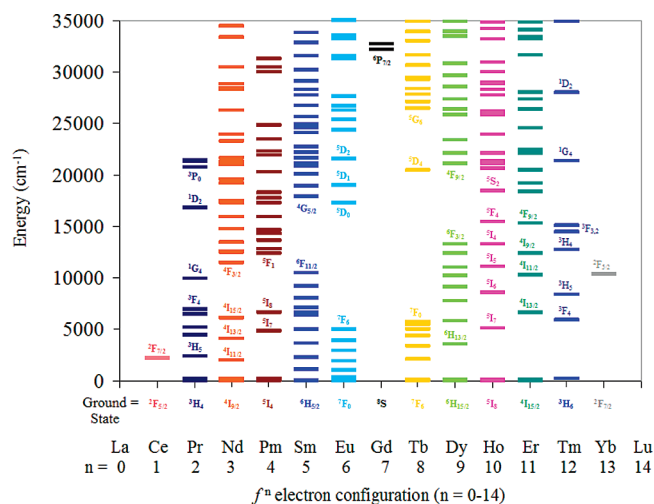
FIGURE 3. A summary of lanthanide excited-state energy levels for the Ln(III) series.
